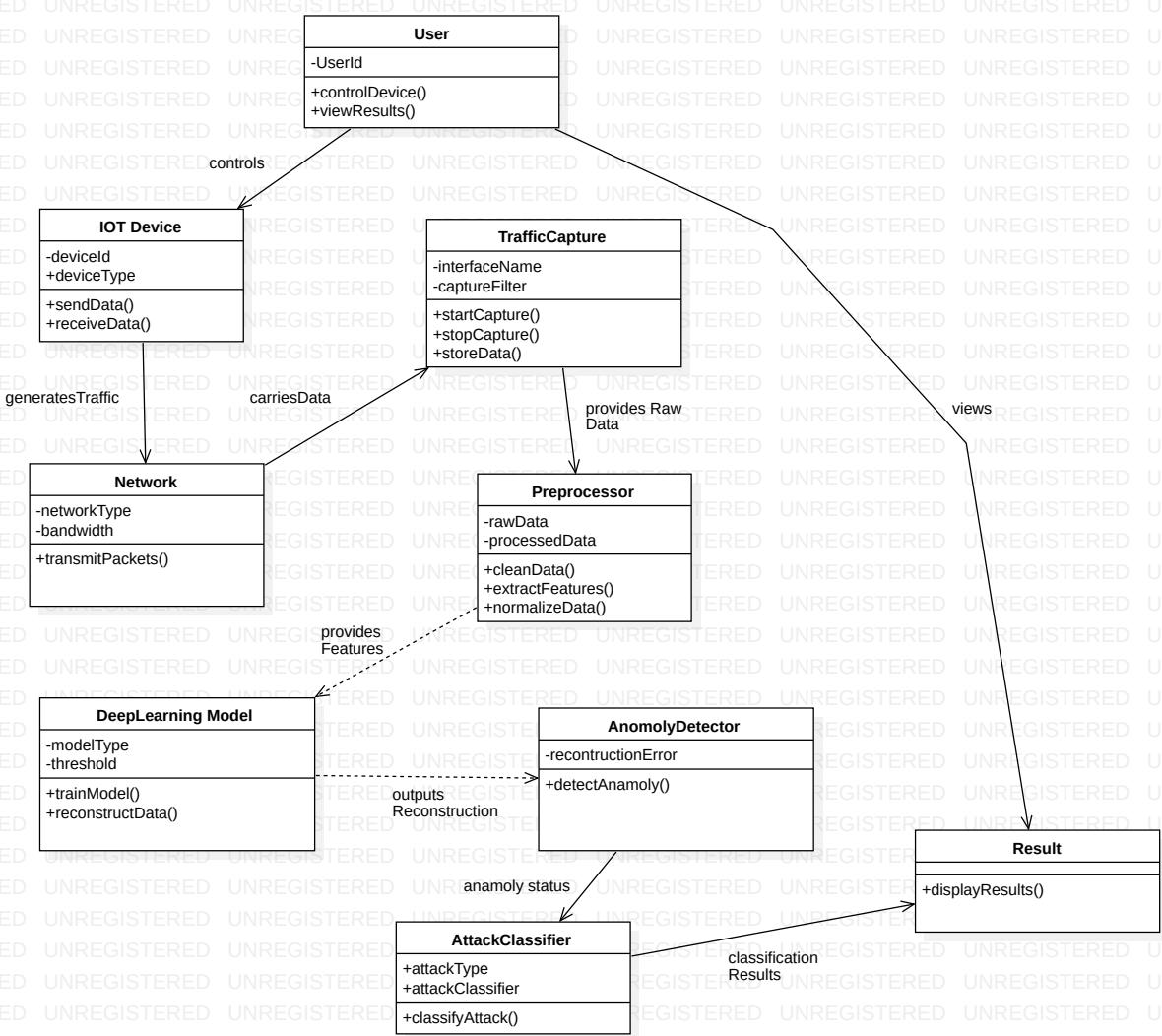
Class Diagram
